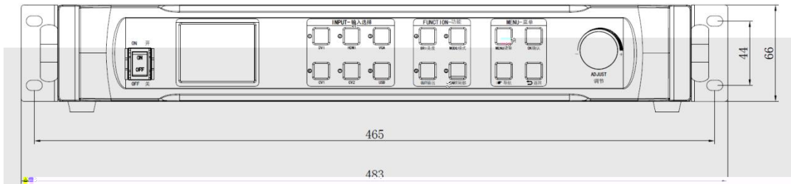
Front panel size drawing
